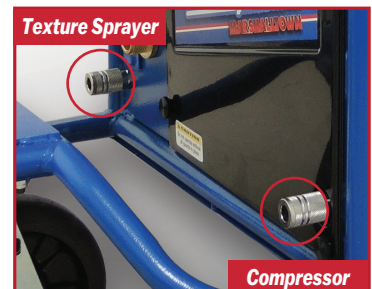
Compressor
