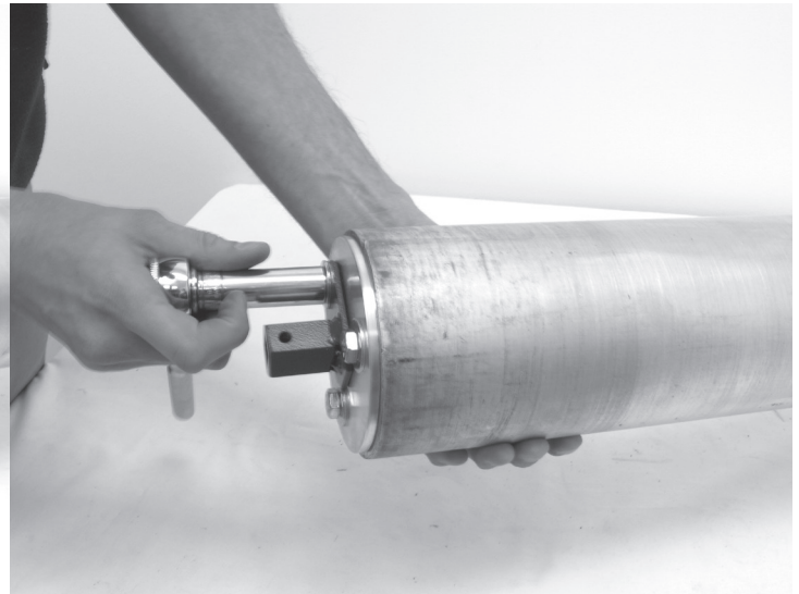
5. Tighten the hex bolts uniformly – perform two or three turns on each bolt and then move on to the next bolt until all bolts are fully tightened. It is important to tighten each hex bolt completely, so the end plugs stay tight in the roller tube. (Use – 9/16" wrench)
