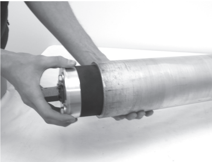
4. Insert power end plug to other side of roller tube. (Parts 1 & 3)
