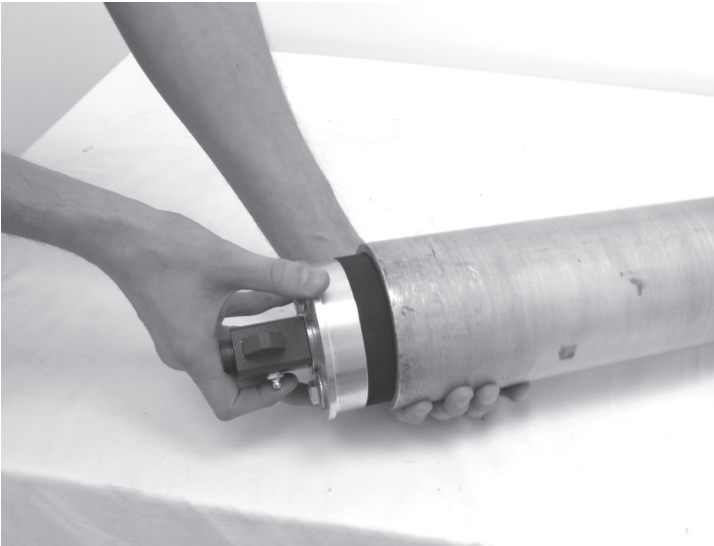
2. Insert lag end plug to one side of roller tube. (Parts – 1 & 2)
