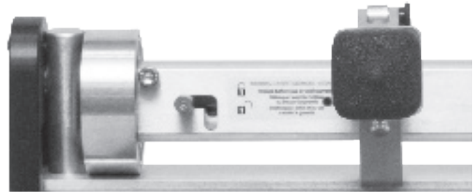
CAM-LOCK IN GESICHERTER POSITION
